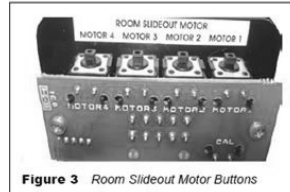
Figure 3 Room Slideout Motor Buttons
