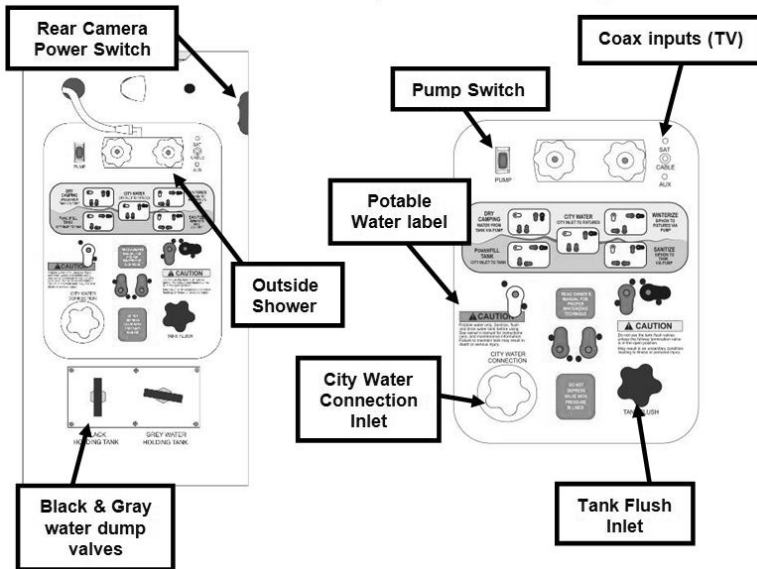
Uni-Dock Utility Center
